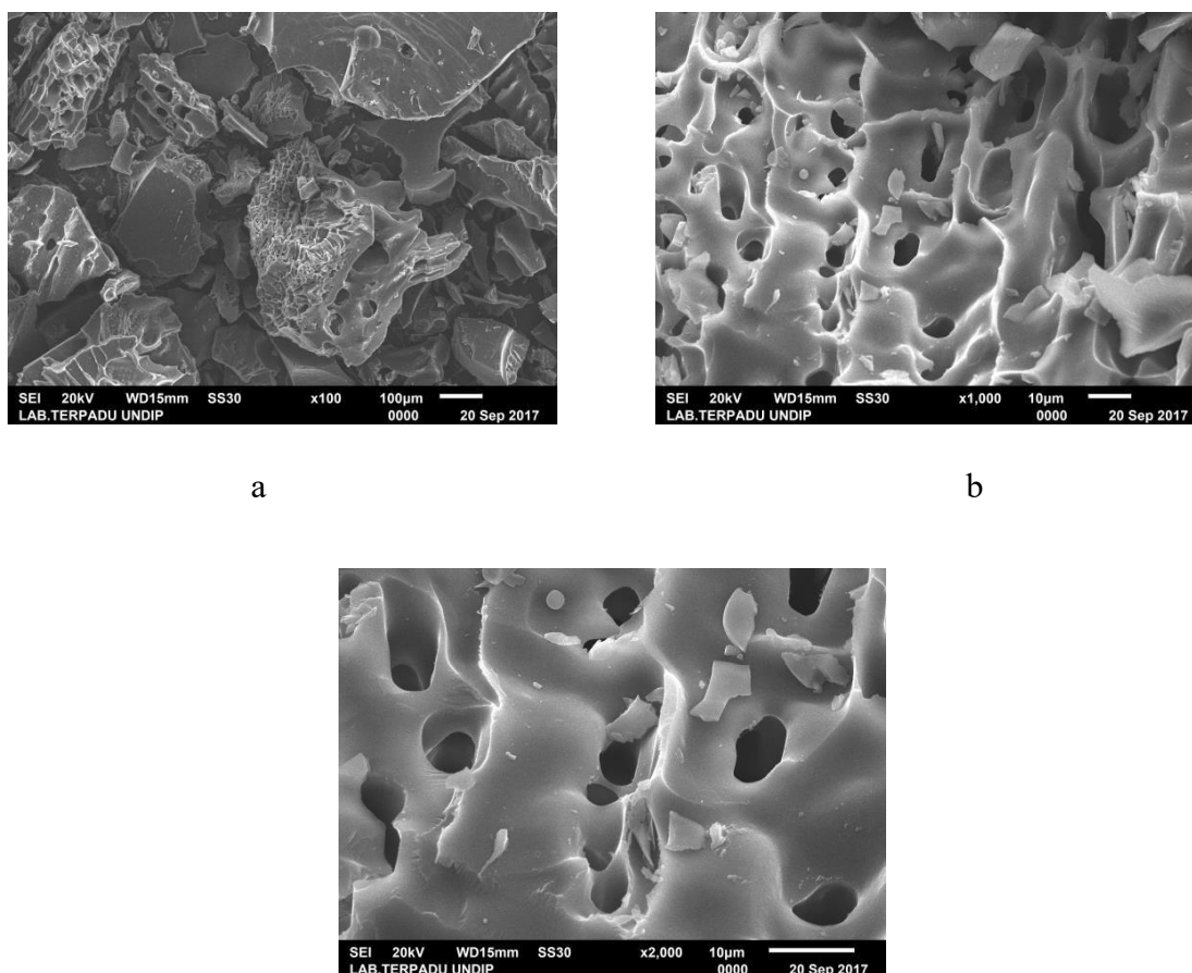
Figure 5. The micrograph of aqueous fraction of Clinacanthus nutans leaf extract microcapsules (a) 100x magnification (b) 1000x magnification (c) 2000x magnification
