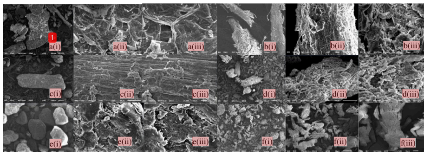
Figure 1. SEM Image of (a) Powder Corn Husk; (b) \alpha -Cellulose; (c) MCC Corn Husk (HCl 2 N); (d) MCC Corn Husk (HCl 4 N); (e) MCC Corn Husk (HCl 6 N); (f) Avicel pH 102; with magnification (i) 100x; (ii) 500x; (iii) 1000x.
