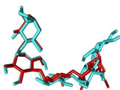
Figure 5. The overlay of the acarbose confirmation before (blue) and after (red) redocking
