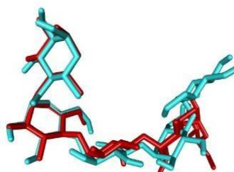
Figure 5. The overlay of the acarbose conformation before (blue) and after (red) redocking
