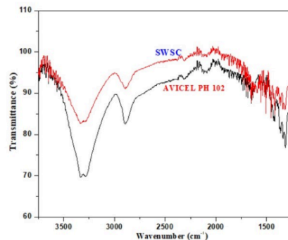
Figure 3. FT-IR Spectrum of Avicel® PH 102 and SWSC
