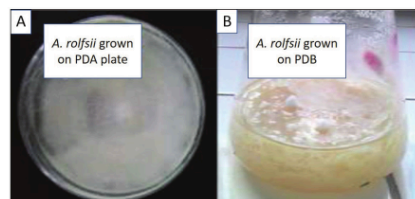
Figure 1: The growth of Athelia rolfsii . Growth on PDA at day 7 (A) and PDB at day 12 at 25°C, five plugs of (A) on PDB agitated at 160 rpm without adding any variations/basal medium (B)
