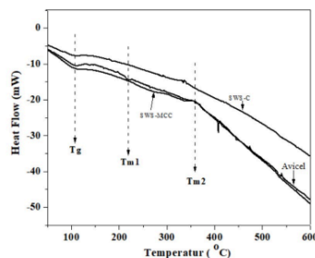
Figure 4: DSC thermograms of SWS-C, SWS-MCC and Avicel
