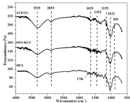
Figure 1: FT-IR spectra of SWS, SWS-MCC and Avicel
