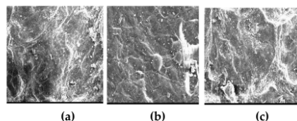
Figure 2. Scanning Electron Microscopy (SEM) of Red Dragon Fruit Stem Starch (a) Soaking Time 1 h, (b) Soaking Time 2 h, (c) Soaking Time 3 h with 1000x Magnification
