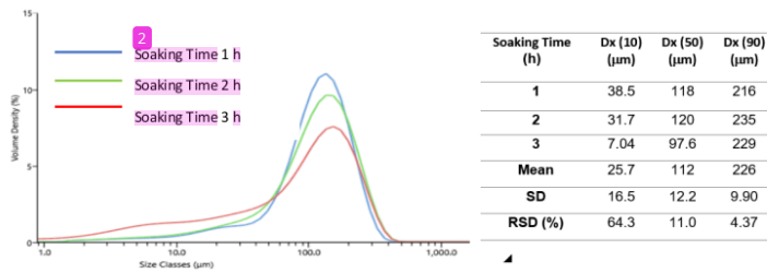
Figure 4. Particle Size Distribution Test Results
