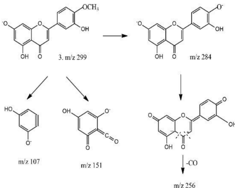
Figure 3. Diosmetin Fragmentation Pattern
