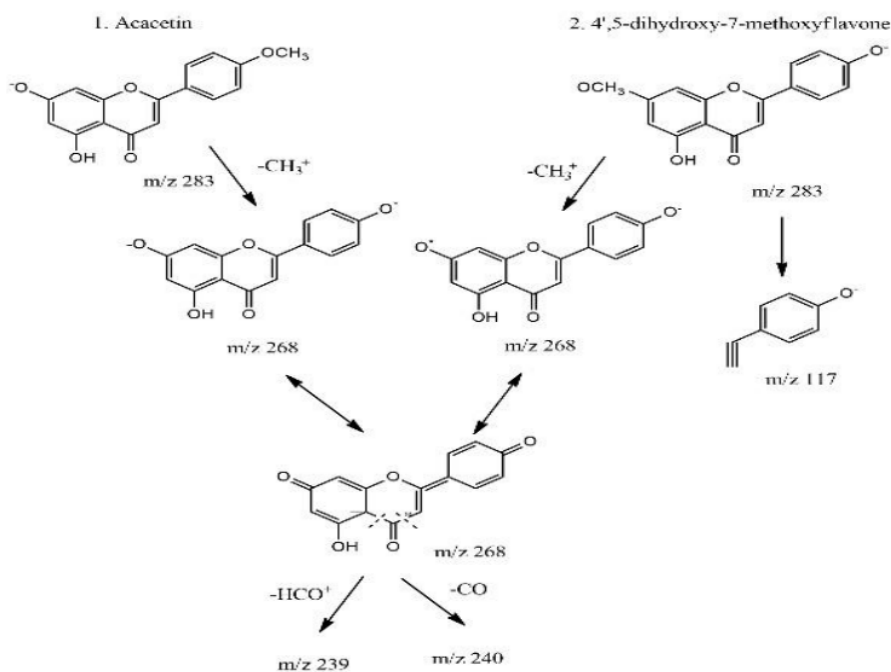
Figure 2. Acacetin Fragmentation Pattern
