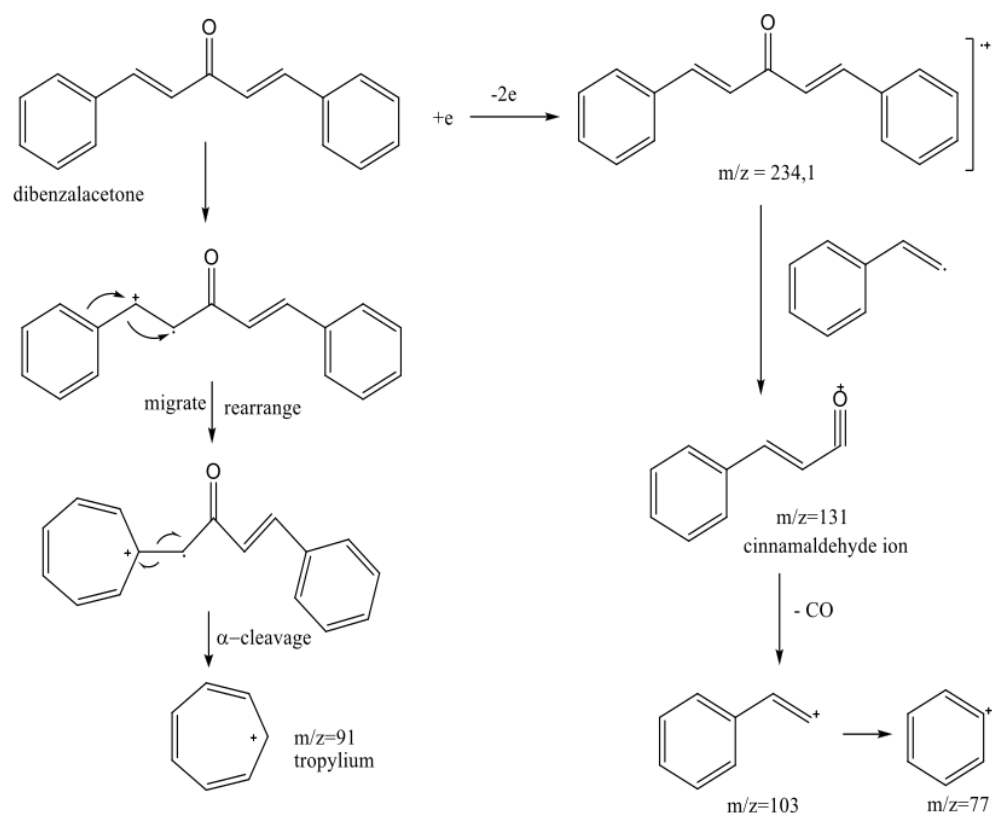
Figure 7. Fragmentation mass spectra of dibenzalacetone.
