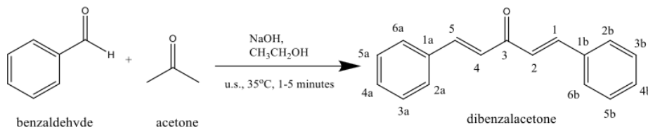
Figure 1. Dibenzalacetone synthesis reaction.
