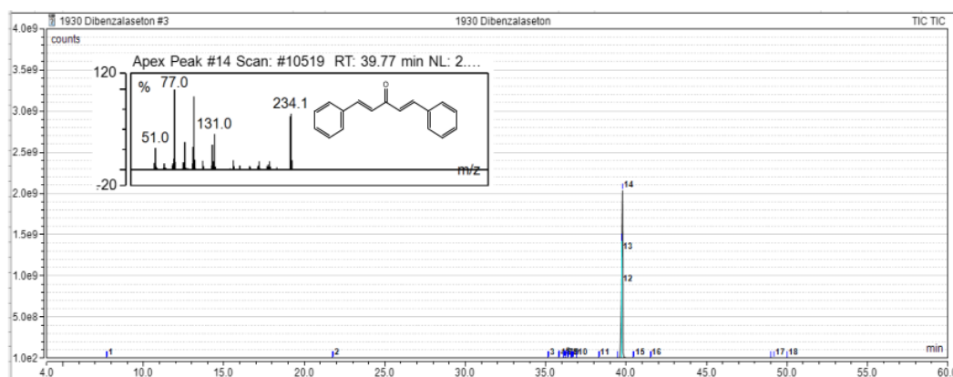
Figure 6. The GC-MS of dibenzalacetone.
