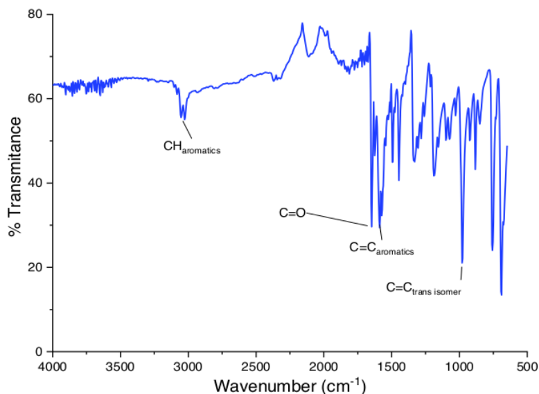
Figure 4. FTIR spectrum of dibenzalacetone.
