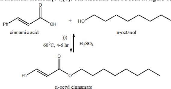
Figure 1. Esterification reaction on cinnamic acid with n-octanol
