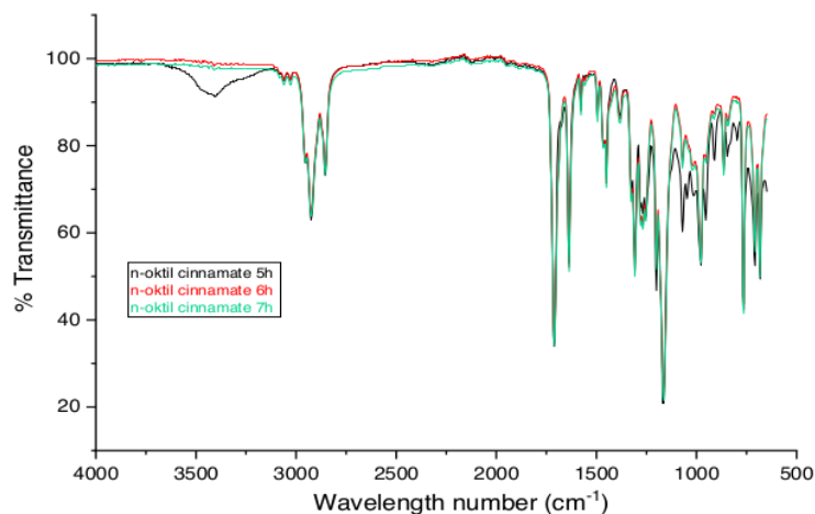
Figure 4. Overlays FTIR n-octyl cinnamate 5,6,dan 7 hours
