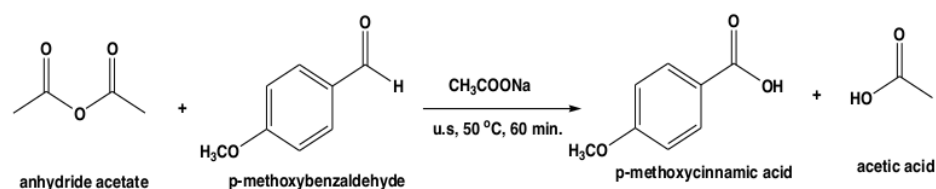
Figure 1. The synthesis of PMCA
