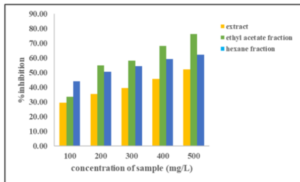
Figure 4. Antioxidants Test of the Sample Using DPPH
