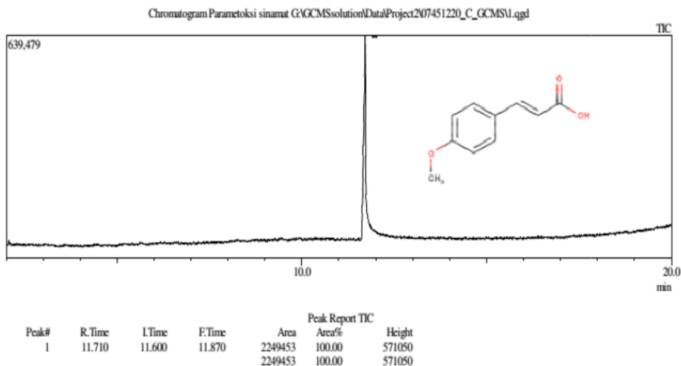
Figure 5. Chromatogram of P -methoxycinnamic Acid Compound
