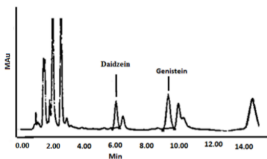
Fig. 2: Chromatogram of soybean samples obtained by HPLC with the Sun Fire TMC-18 C18 column (150 mm x 4.6 mm, 5 \mu m). The mobile phase used was methanol: 0.1% acetic acid (53:47), flow rate of 1.0 ml/min
