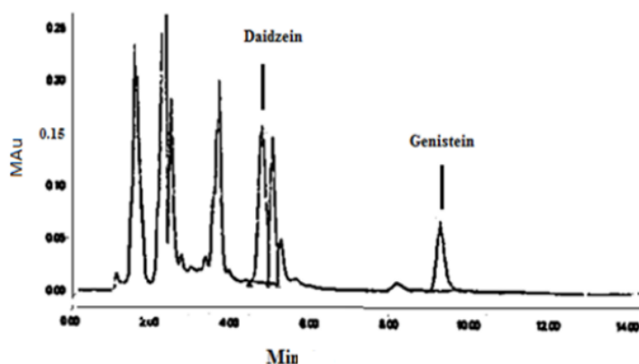
Fig. 1: Chromatogram of soybean samples obtained by HPLC using sun fire TMC-18 C18 coloumn (150 mm x 4.6 mm, 5 µm). The mobile phase used was acetoniiril: 0.1% acetic acid (35: 65), flow rate of 0.8 ml/min
