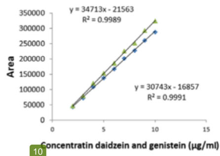
Fig. 4: The relationship between the concentration of daidzein and genistein (x-axis) and peak area (y-axis)
